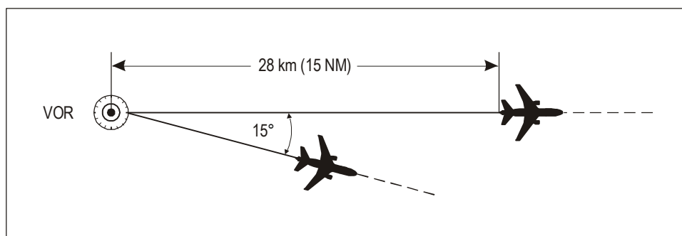
Figure 5-4. Separation using the same VOR (see 5.4.1.2.1.2 a))
