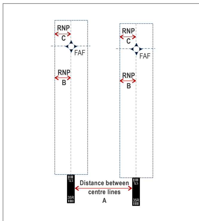
Figure 6-2. RNP value and distance between centre lines
