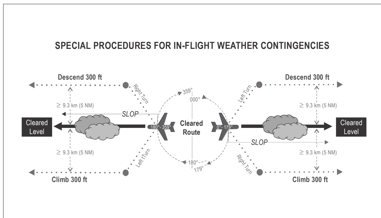
Figure 15-2. Visual guide for weather deviation procedures if a revised ATC clearance cannot be obtained (see 15.2.4.3)
