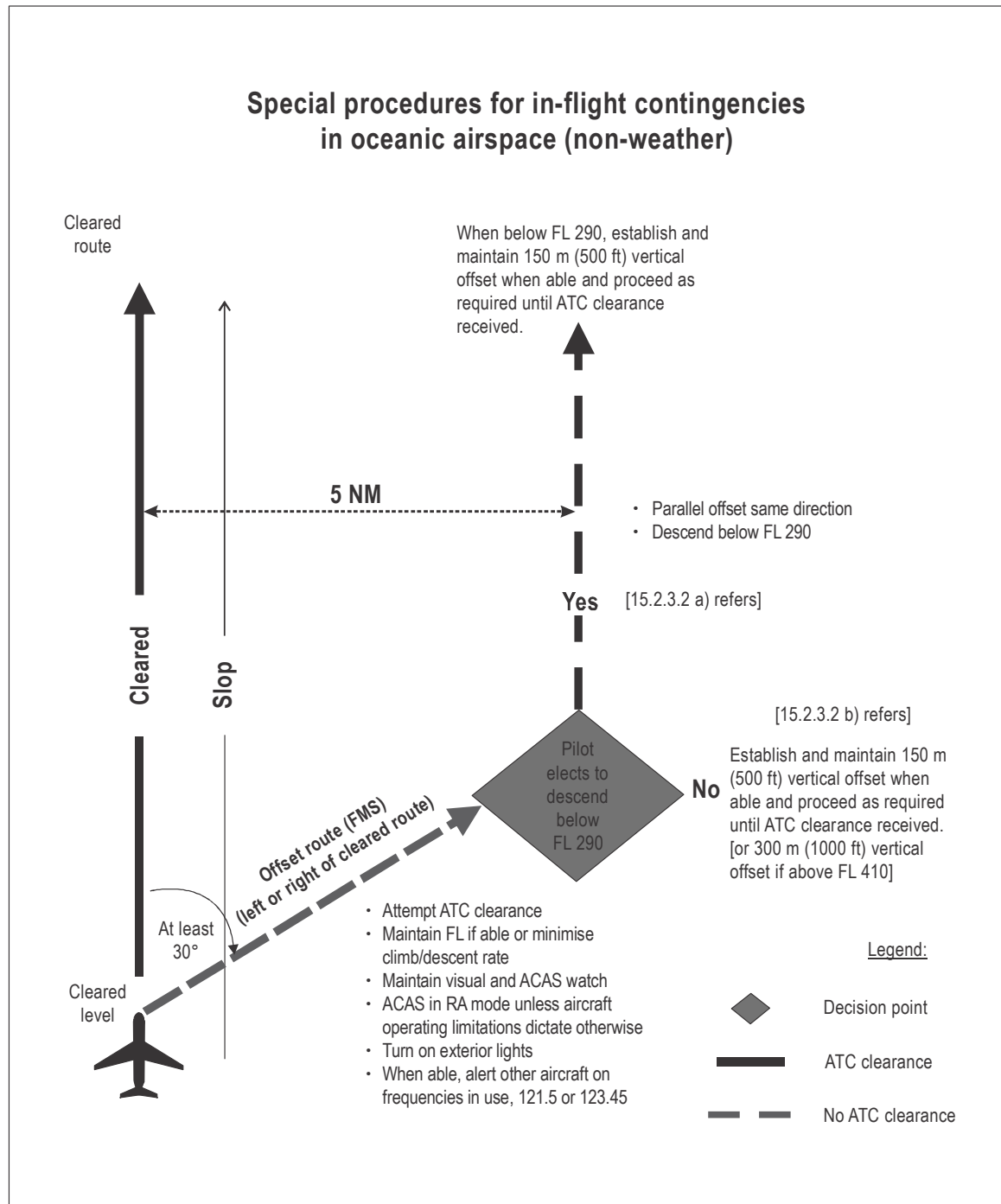
Figure 15-1. Visual guide for contingency procedures (see 15.2.2 and 15.2.3)
